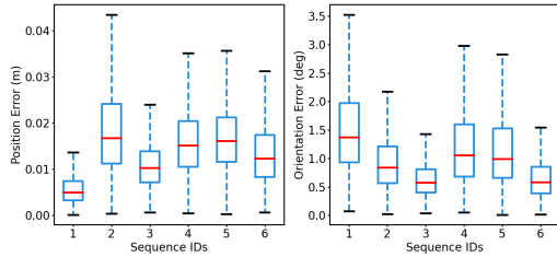
Figure 5. Error distribution of event-based CPR results achieved by PEPNet using a random split. (a) Translation errors. (b) Rotation errors.
